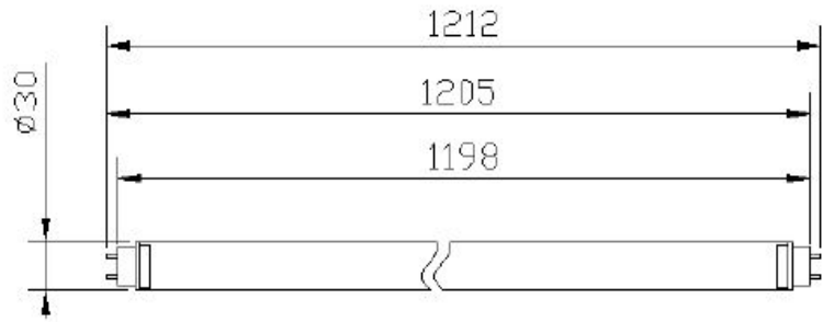
T8 tube Dimension Diagram (unit: mm)
